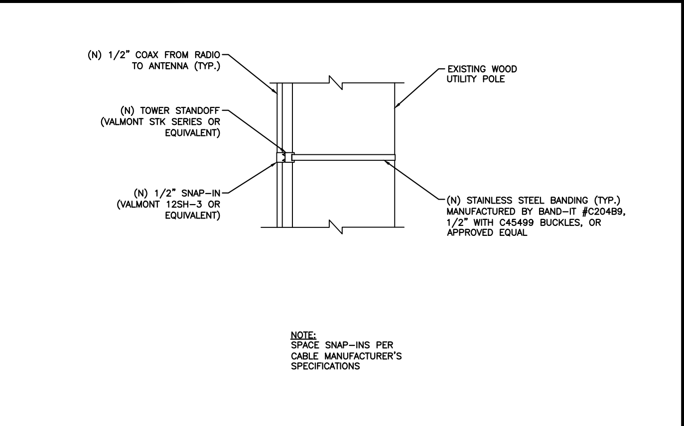
CABLE MOUNTING DETAIL SCALE: NOT TO SCALE 2
