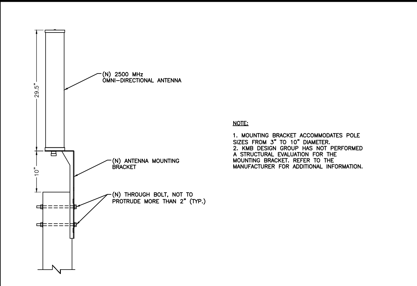
ANTENNA MOUNTING DETAIL SCALE: NOT TO SCALE 3
