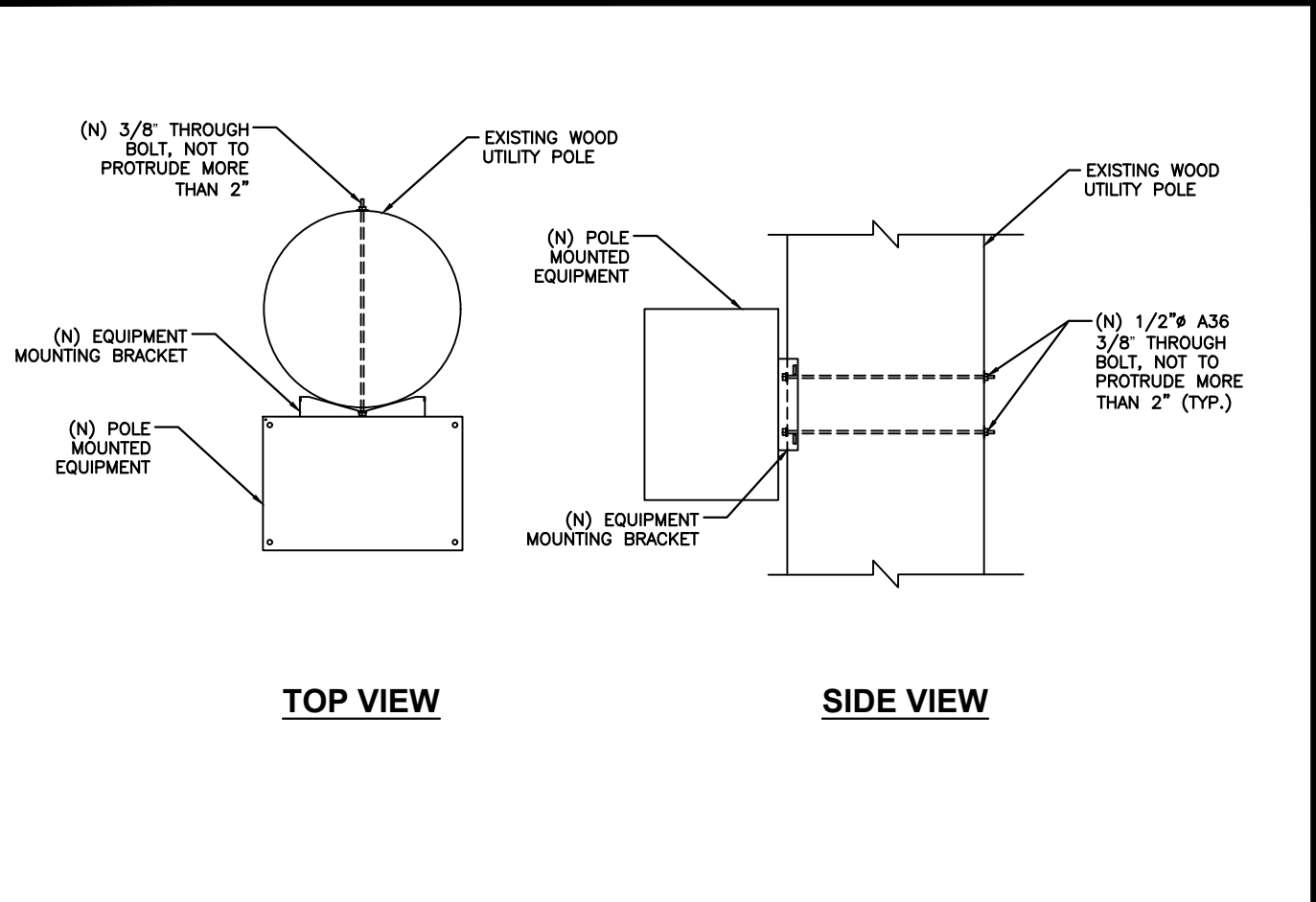
EQUIPMENT MOUNTING DETAIL SCALE: NOT TO SCALE 1
