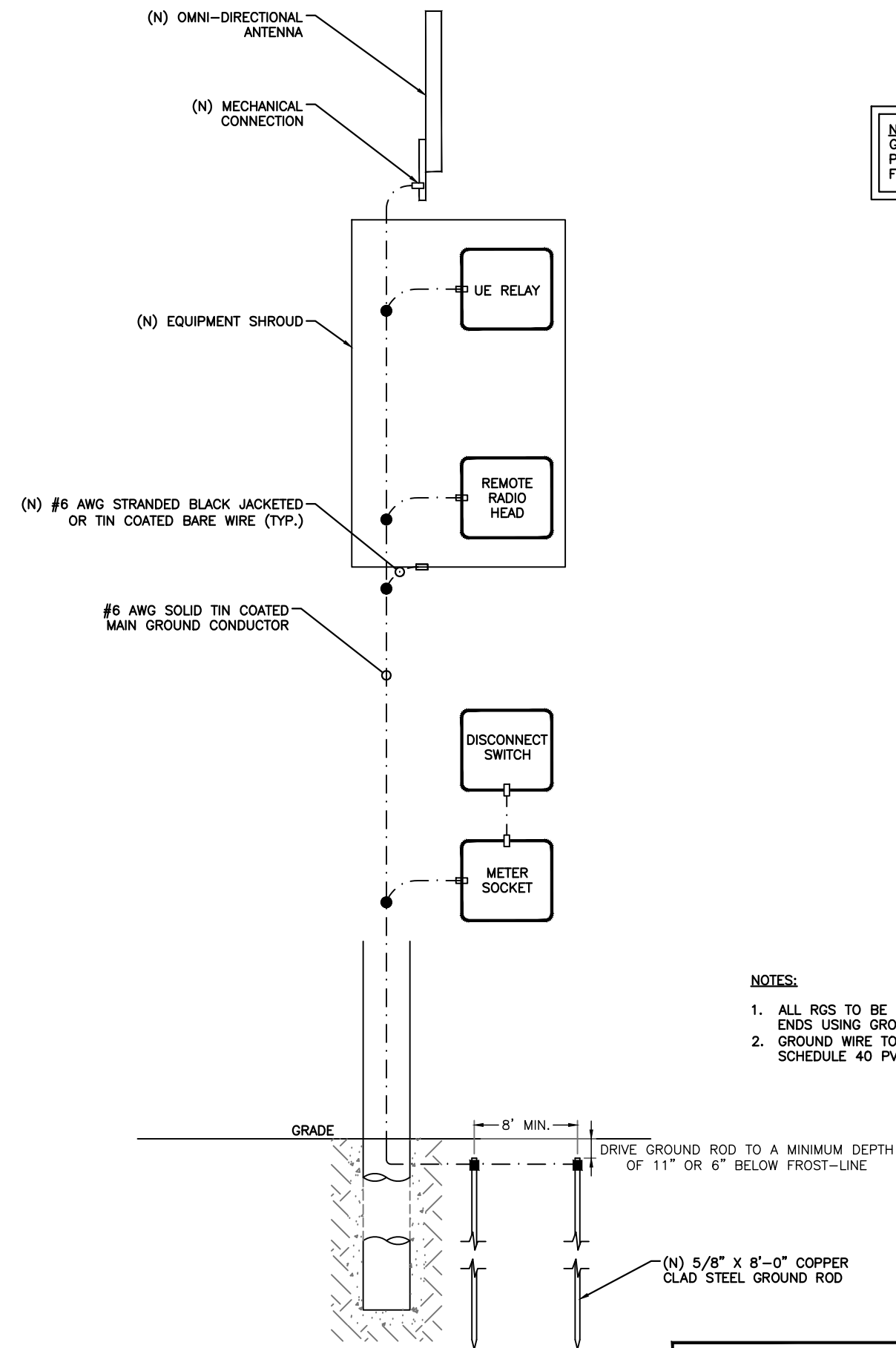
GROUNDING RISER DIAGRAM SCALE: NOT TO SCALE 3
