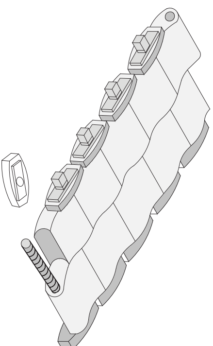
CALPICO LINX PRIOR TO TIGHTENING DETAIL "C" NOT TO SCALE
