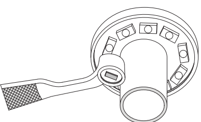
TIGHTENING TO FORM AIRTIGHT & WATERTIGHT SEAL DETAIL "D" NOT TO SCALE
