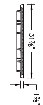
FRAME & STANDARD CAMBRIDGE NETWORK SOLUTIONS (CNS) COVER ASSEMBLY DETAIL NOT TO SCALE
