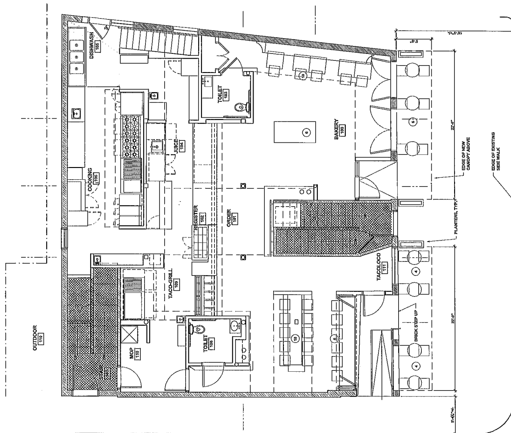
1 FIRST FLOOR FURNITURE & FINISH PLAN
