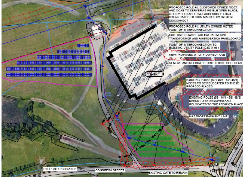
1 SITE PLAN - 0 CONGRESS ST, WOBURN, MA: 660.53 kWDC PV SYSTEM NOT TO SCALE
