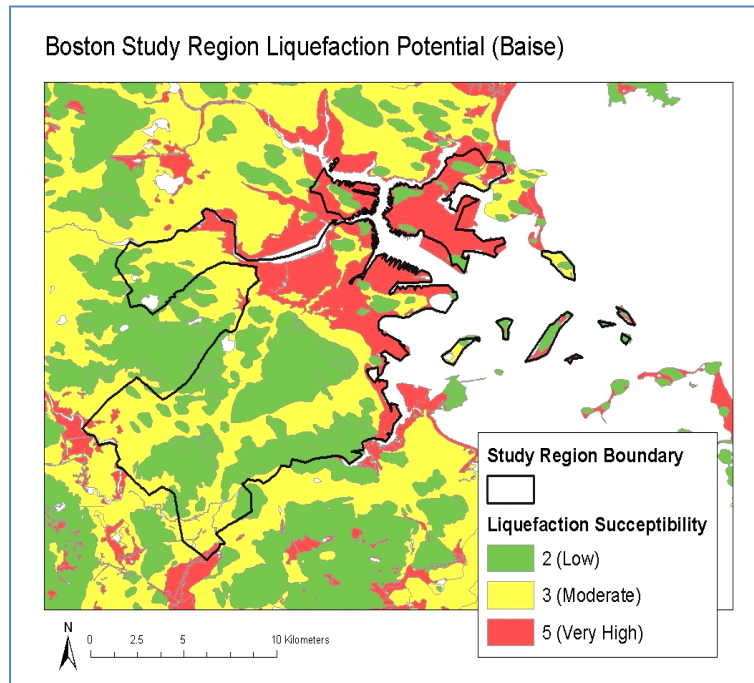
Figure 2. Boston Study Region Liquefaction Potential
