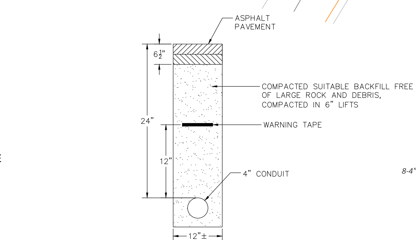
ROADWAY PATCH AND DUCT BANK INSTALLATION DETAIL
