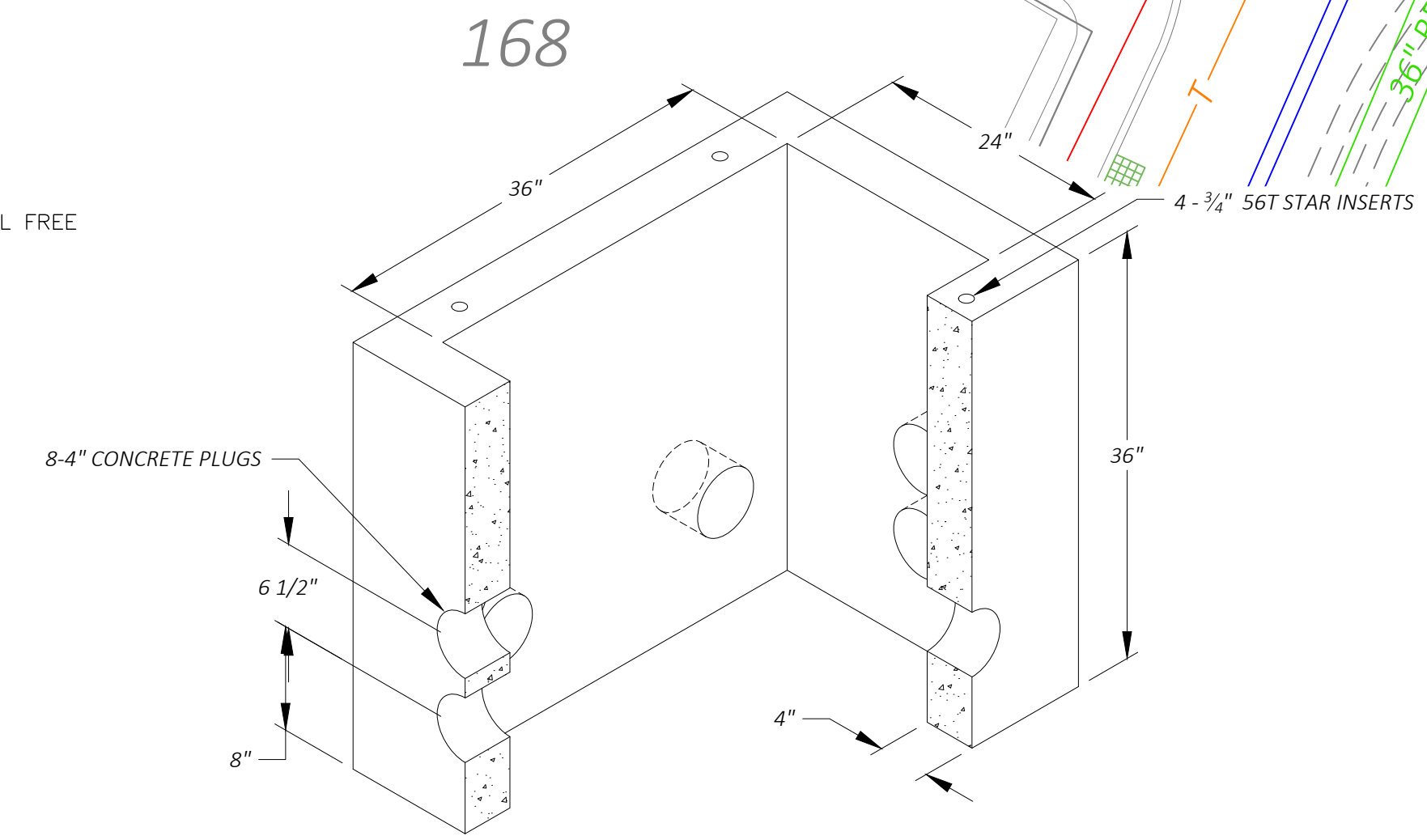
TYPICAL 24" X 36" X 36" HANDHOLE
