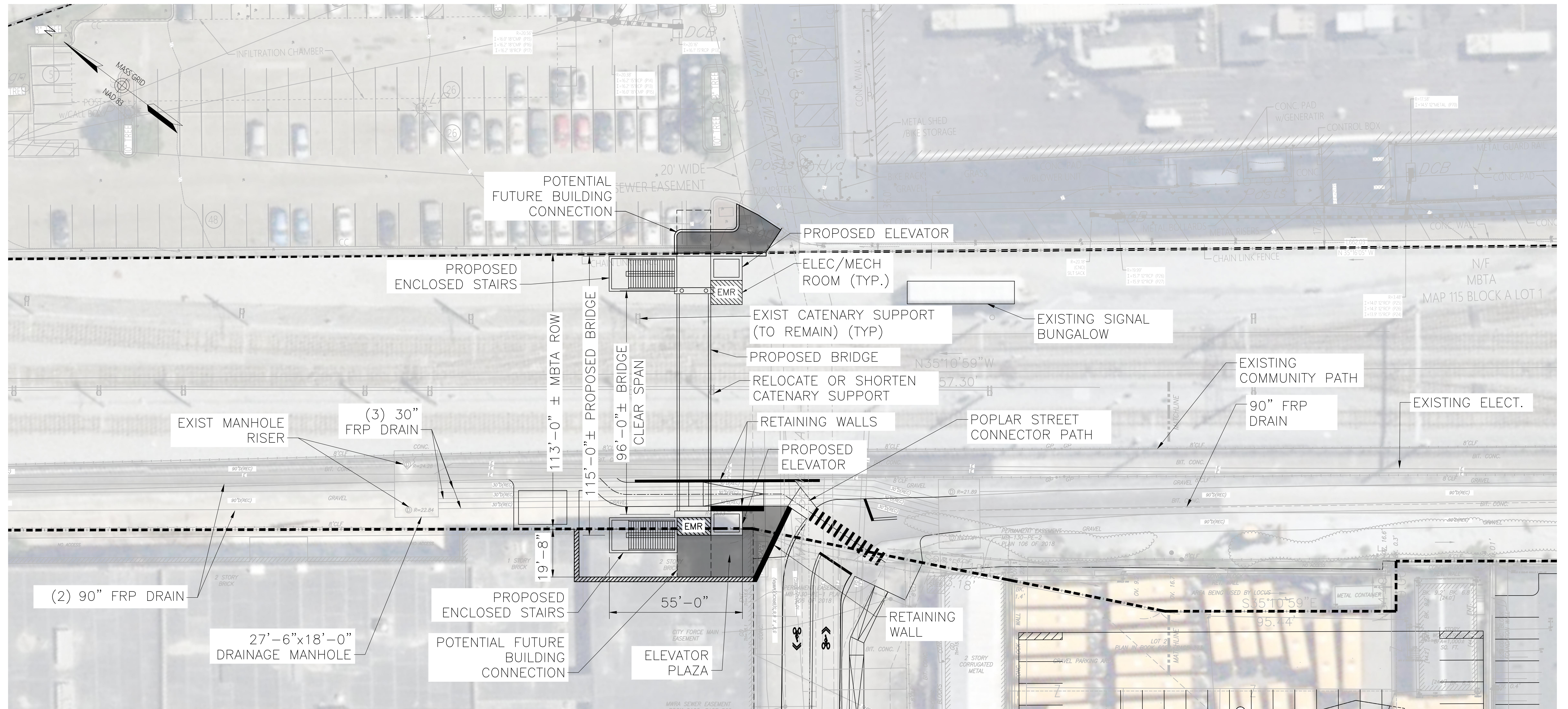
PEDESTRIAN BRIDGE PLAN SCALE: 1" = 20'
