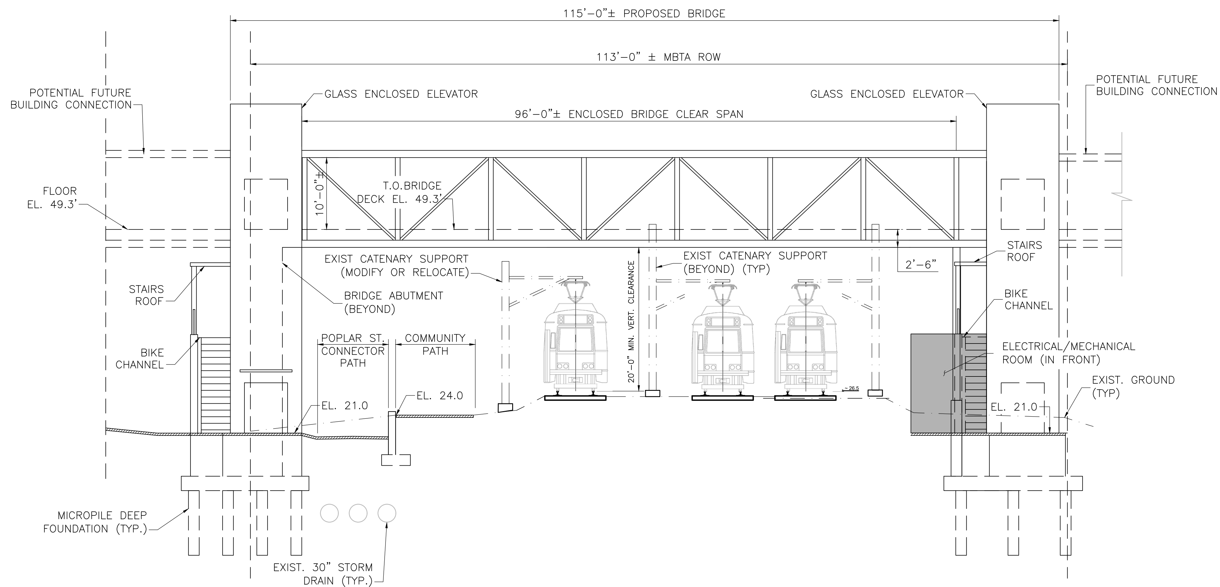
PEDESTRIAN BRIDGE ELEVATION (LOOKING NORTH)
