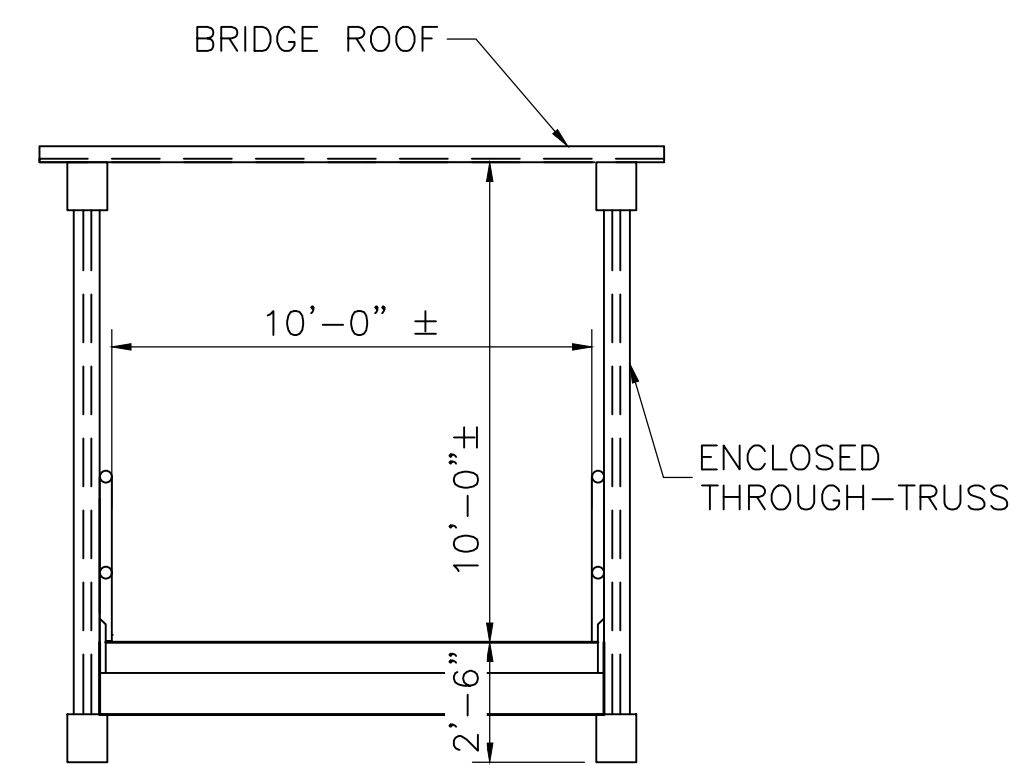
PEDESTRIAN BRIDGE TYPICAL SECTION
