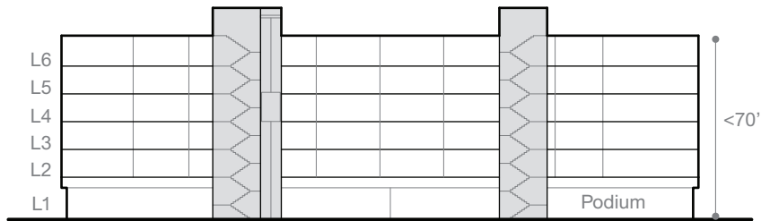
Building Section
