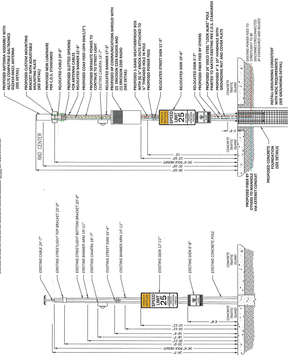
② EXISTING PROFILE - REAR VIEW LOOKING SOUTHWEST TOWARD BROADWAY
